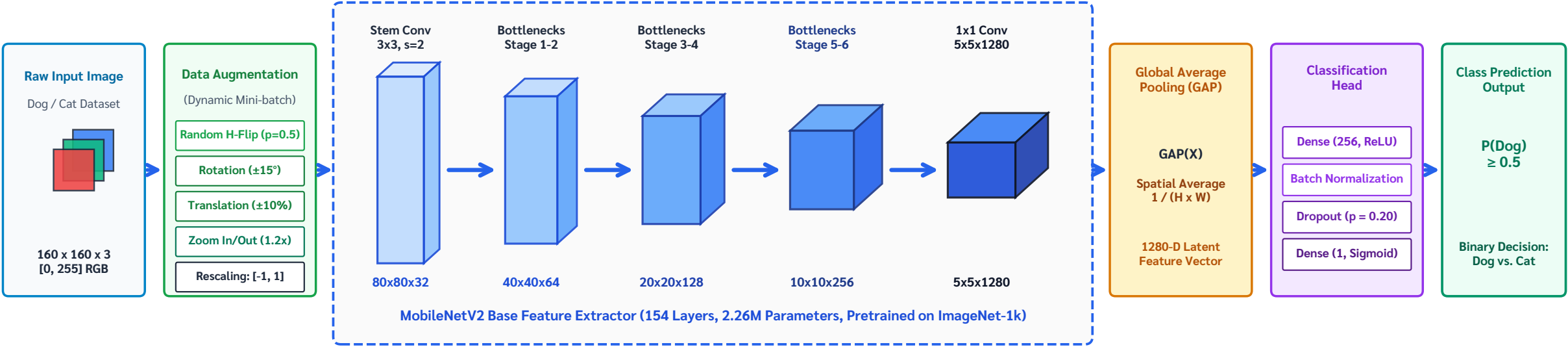
Figure 2(a): End-to-End Transfer Learning Computational & Tensor Pipeline
